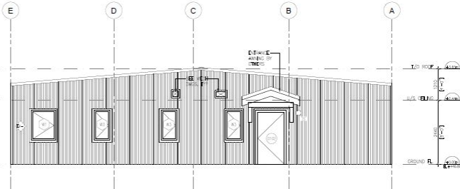
3 EXTERIOR ELEVATION: WEST A300 1/8"
