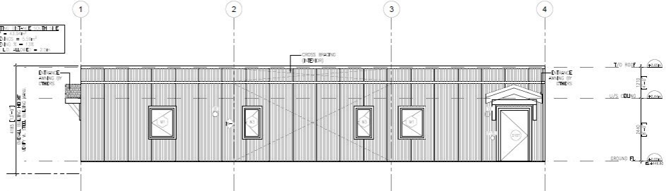
2 EXTERIOR ELEVATION: SOUTH A300 1/8"
