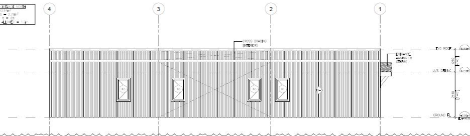
1 EXTERIOR ELEVATION: NORTH A300 1/8"
