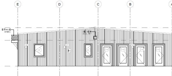
4 EXTERIOR ELEVATION: EAST A300 1/8"
